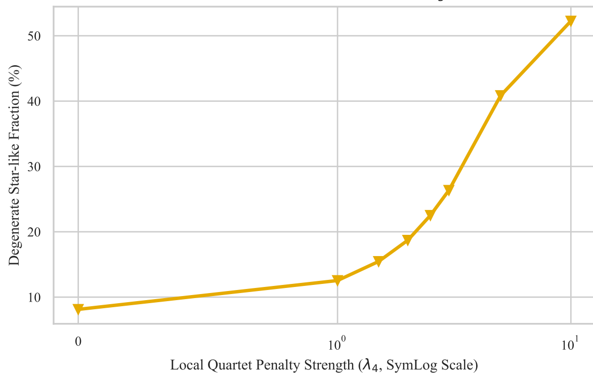
(A) Phase 2 Star-Loophole Generation ( \lambda_g = 0.0 )
