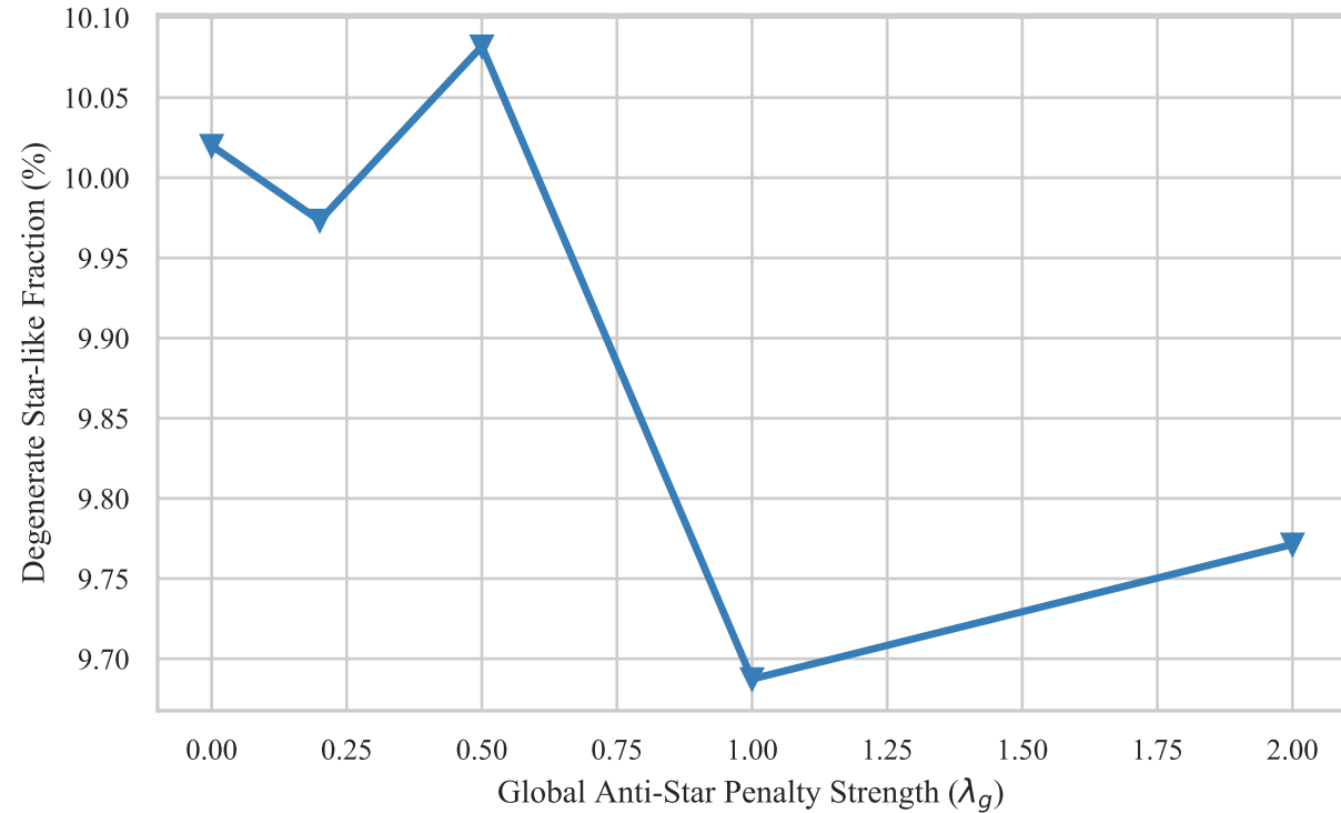
(C) Phase 3 Star Response under Gridlock ( \lambda_4 = 2.0 )
