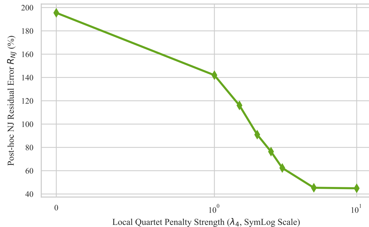
(B) Phase 2 Macro-Topological Distortion
